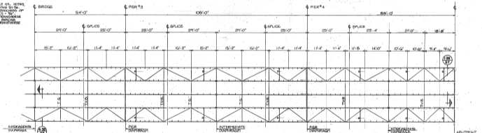
BRACING PLAN - E BRIDGE TO E ABUTMENT 7'-10" 0"
