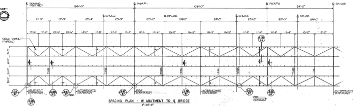
BRACING PLAN - W ABUTMENT TO E BRIDGE 7'-10" 0"
